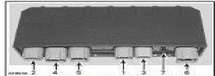
TYPICAL — BOMBARDIER 290 W MPEM — RET MODELS 1. High tension coil, 4-DC housing 2. Generating coils low and high speed and trigger coil, 4-DC housing 3. Air temperature sensor, 4-DC housing 4. Trigger coils, 4-DC housing 5. DESS pre-amp, 4-DC housing 6. Reverse switch and alarm, DESS pre-amp and ignition coil switch, 4-DC housing 7. Air temperature sensor, 4-DC housing 8. Atmospheric pressure input
