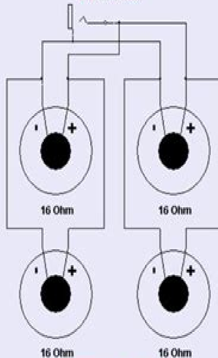
PARALLEL WIRING
