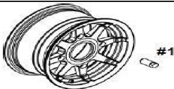
Aluminum Wheel (LE Models) 30 ft. lbs. + 90° (1/4 turn)
