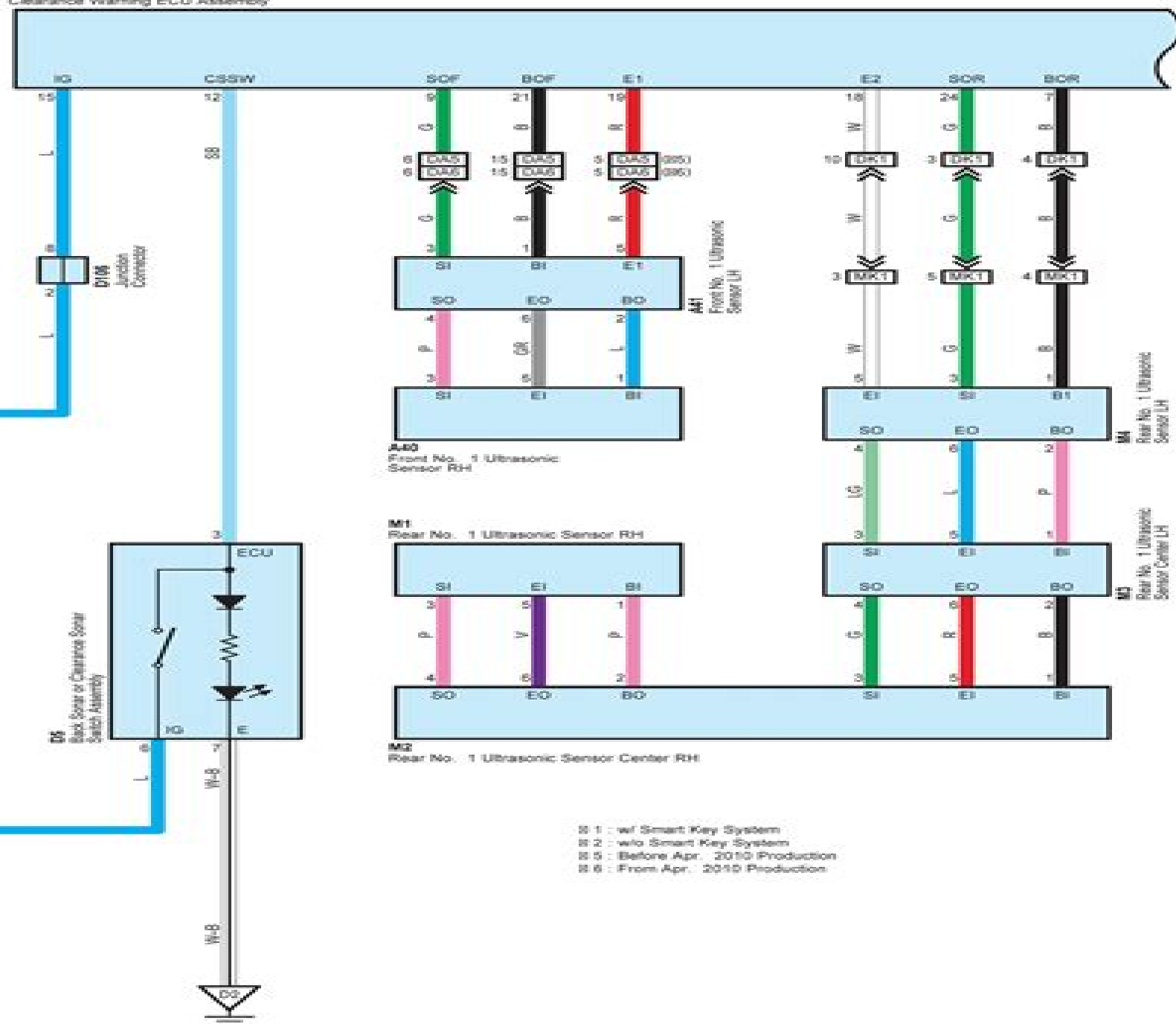
D17 Clearance Warning ECU Assembly
