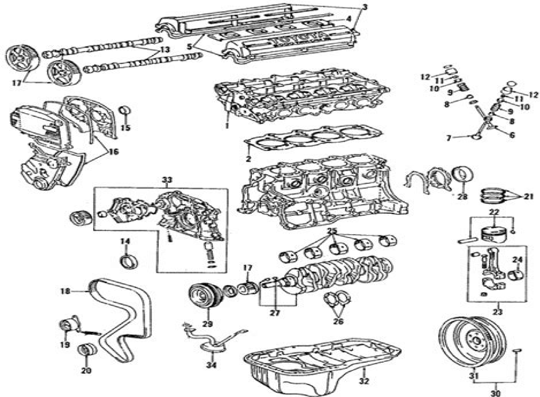
ENGINE - GAS, 4 CYLINDER, 1.6L & 1.8L D.O.H.C.
