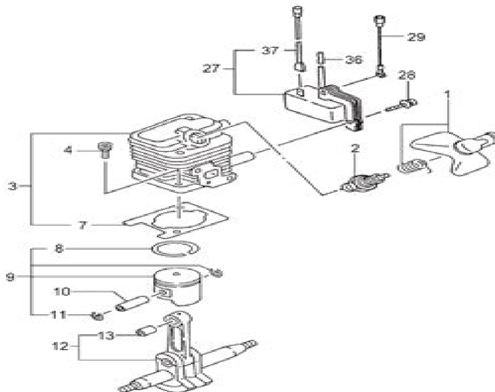
CYLINDER, PISTON, CRANKSHAFT - FIGURE 1
