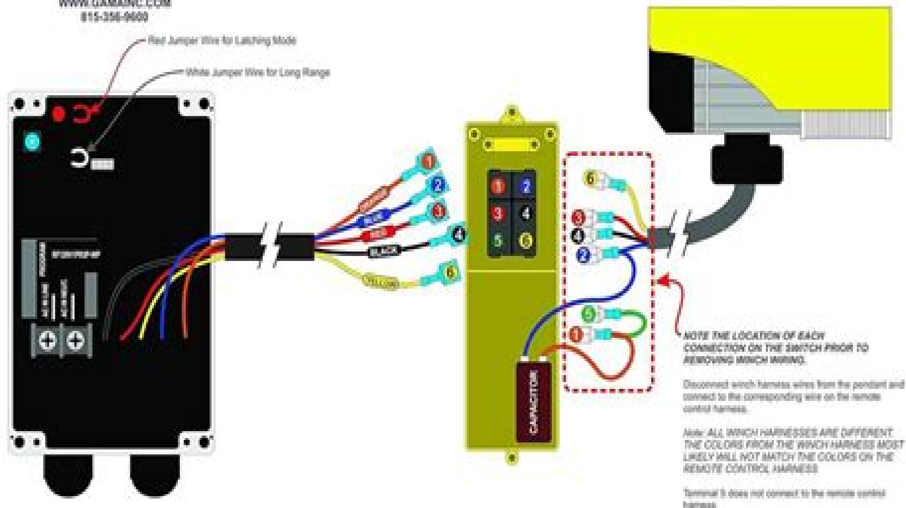
RF120V1PR3P-WP Pendant Wiring for Winches With Capacitor in Pendant
