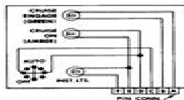
CRUISE CONTROL INST. PANEL SW.
