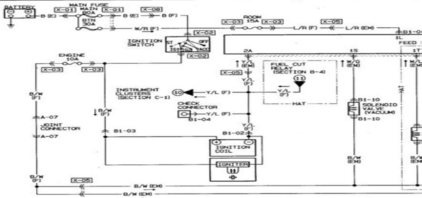
B1-01 FEED BACK CARBURETOR CONTROL UNIT (EM)
