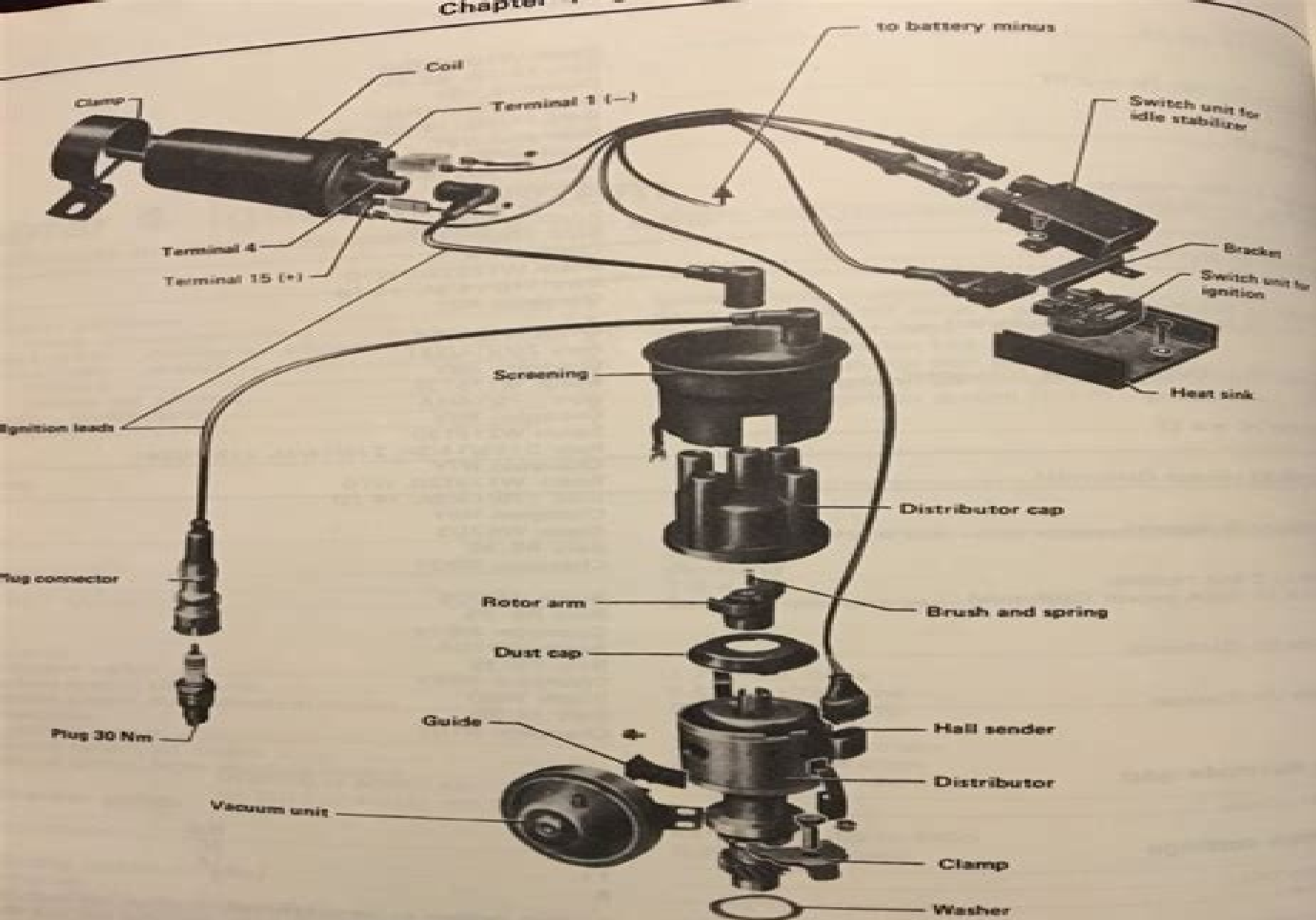
Fig. 4.1 Transistorized ignition components (Sec 1)
