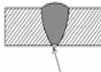
Incomplete Penetration
