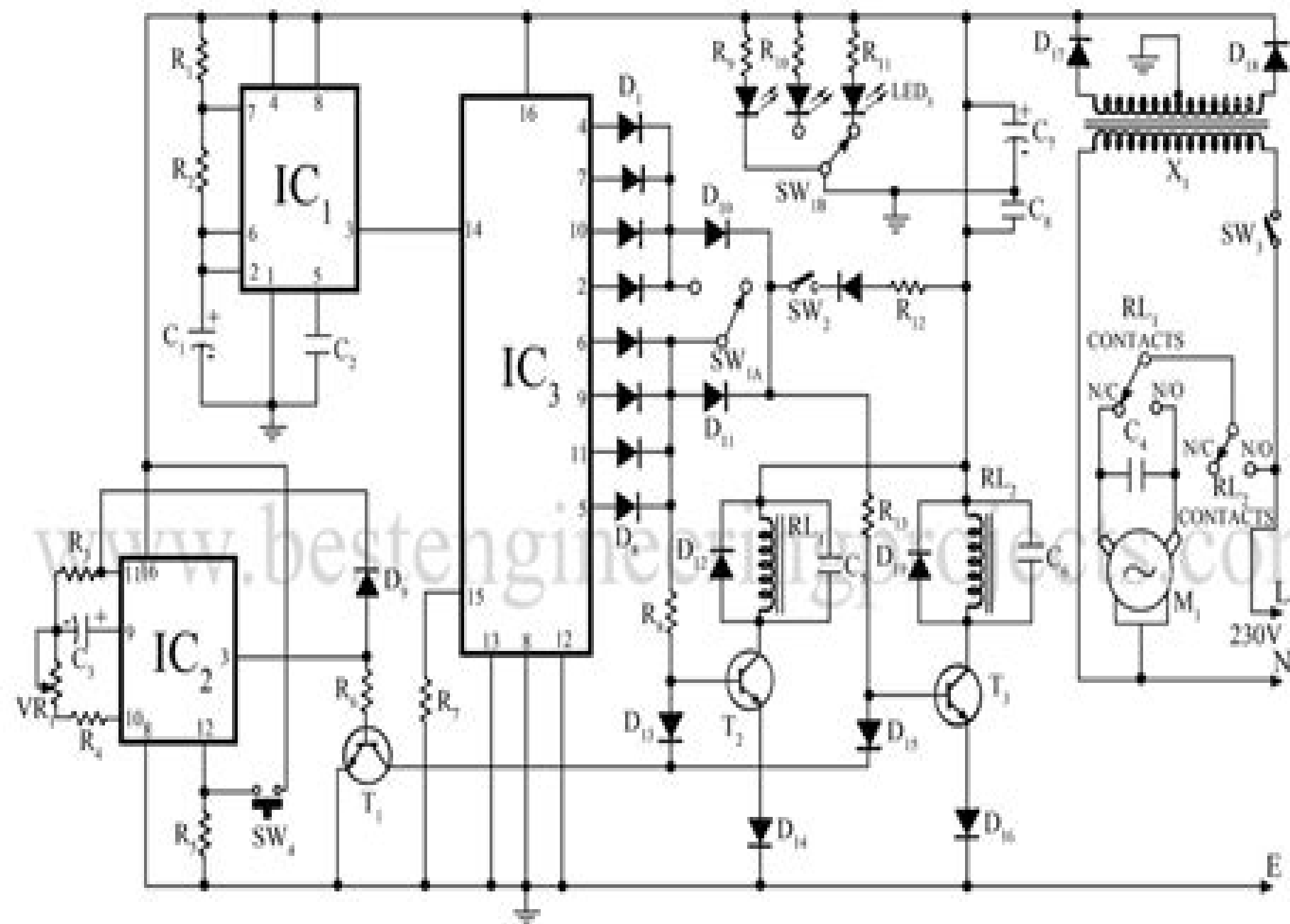
Figure 1 Circuit Diagram of Electronic Washing Machine Control
