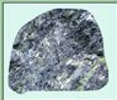
Blue schist
