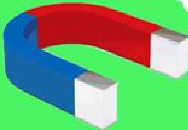
Permanent Magnet
