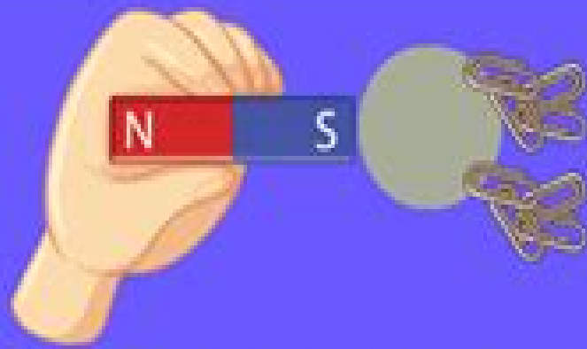
Temporary Magnet
