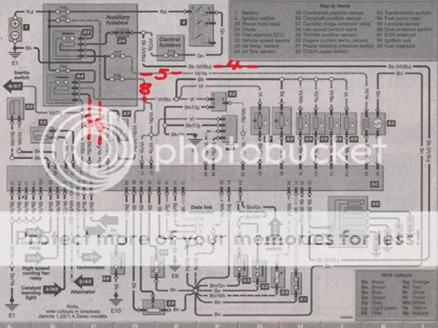
Diagram 6: Typical petrol engine management up to Feb 2000
