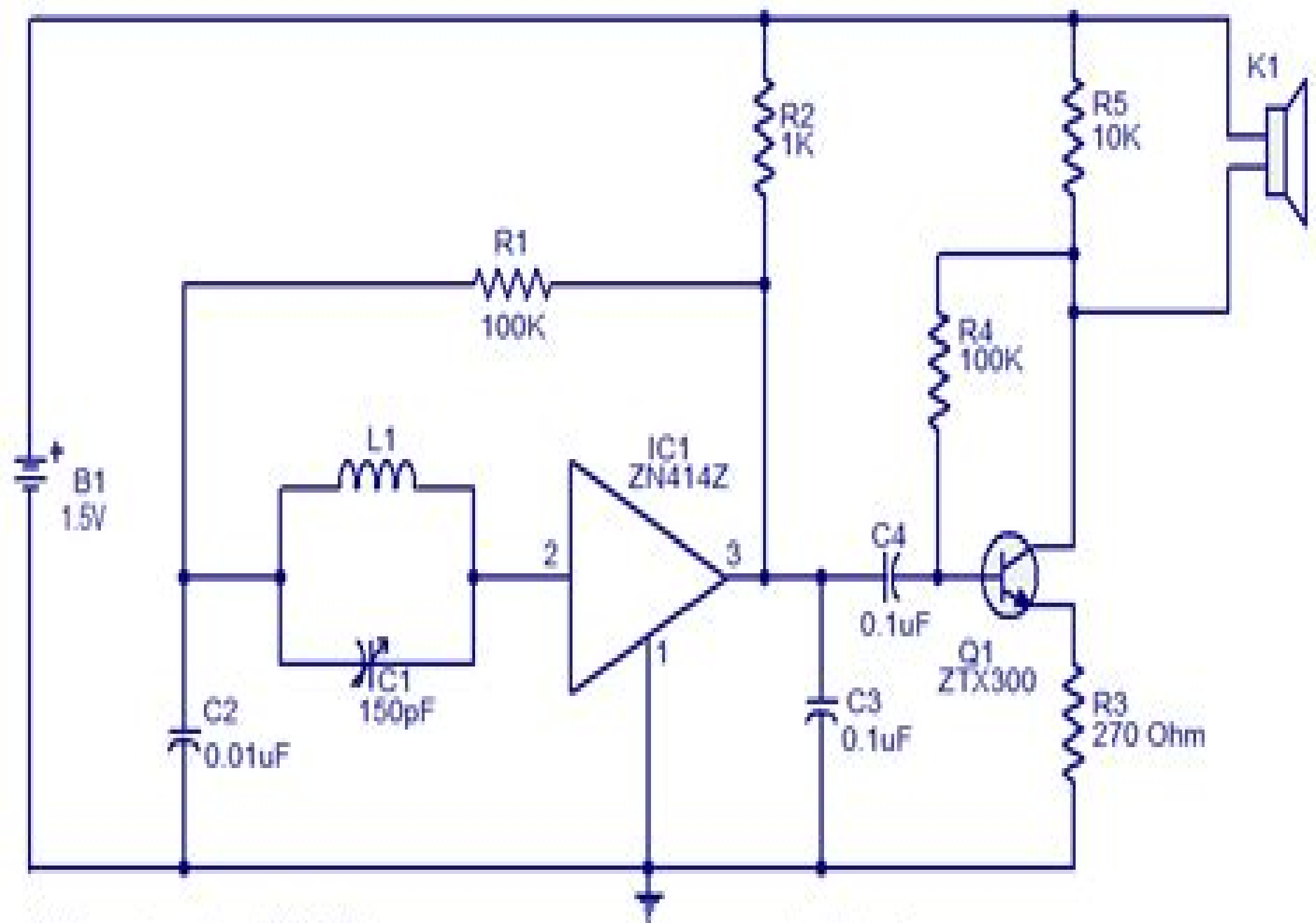
AM receiver using ZN414Z
