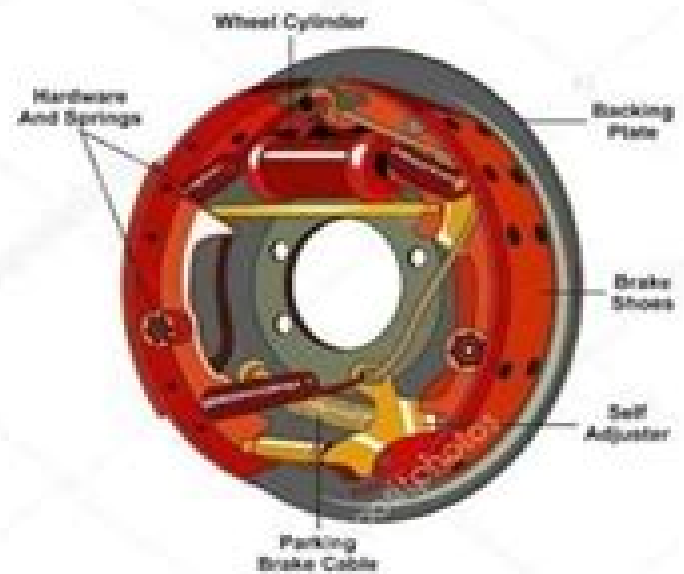
Drum Brake
