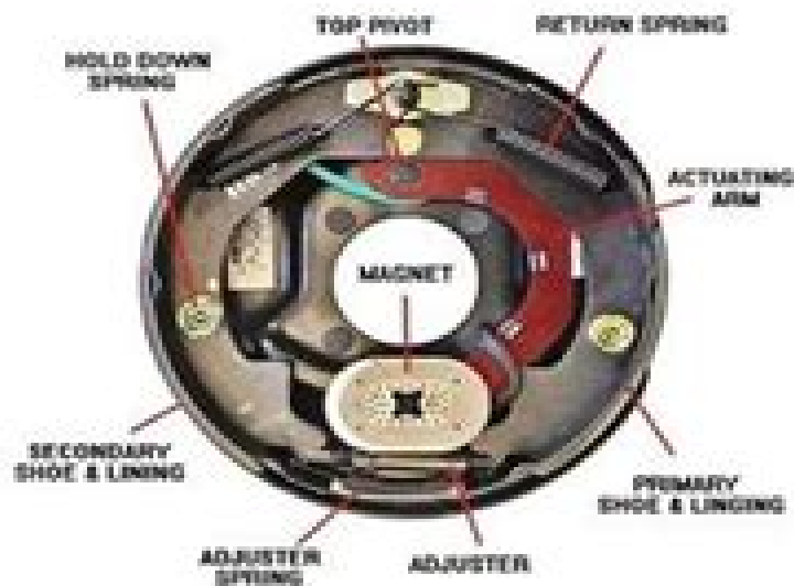
Electric Brake
