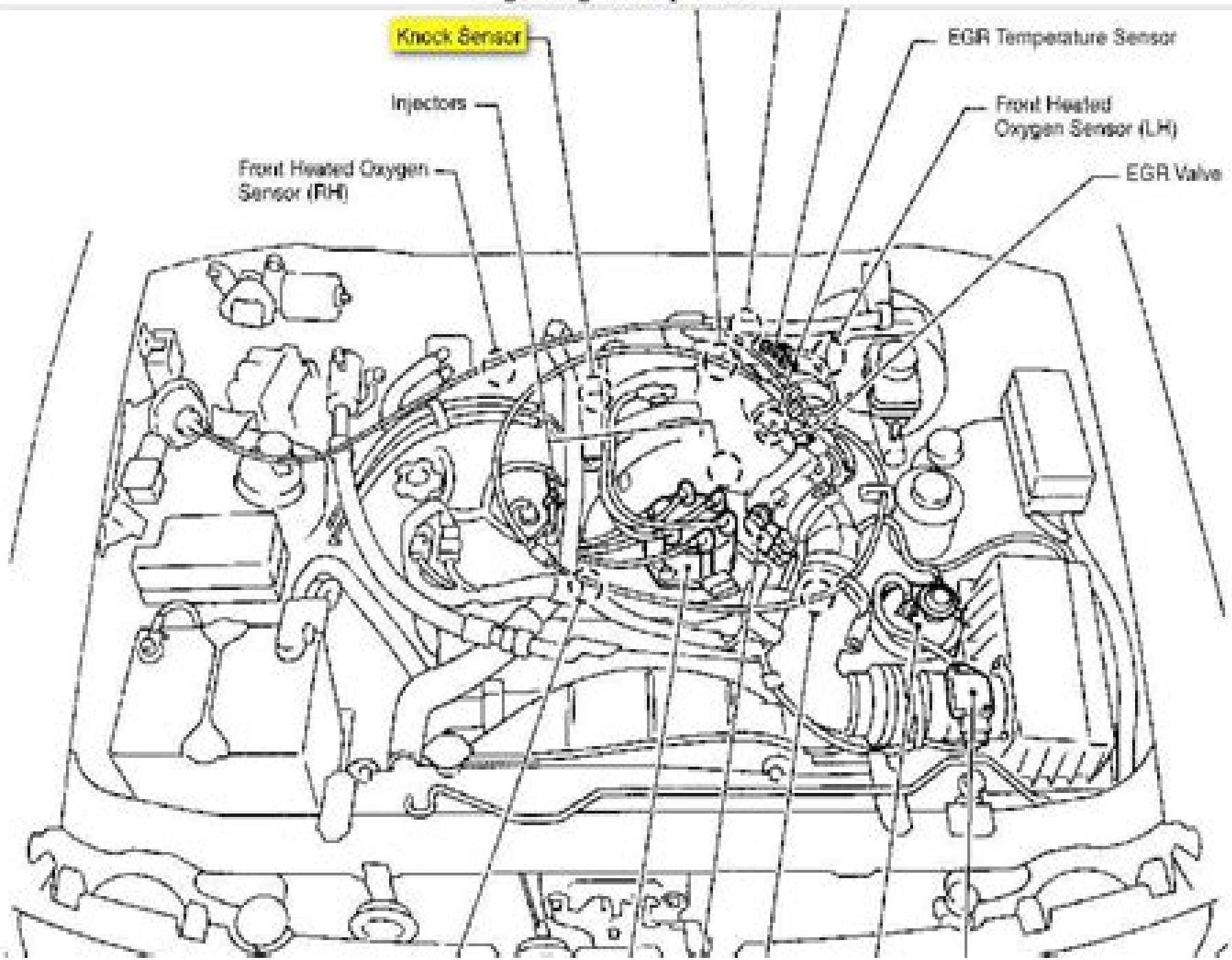
Fig. 2: Engine Compartment
