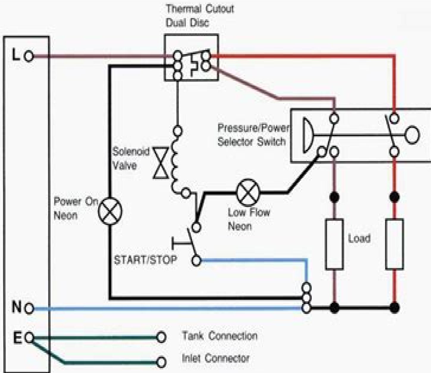
Internal Wiring Diagram
