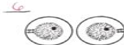
Cytokinesis
