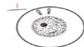
Interphase
