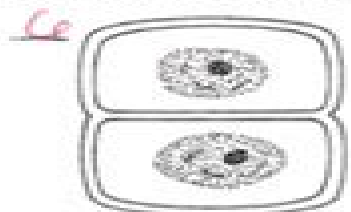
Cytokinesis
