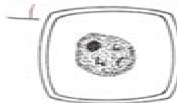
Interphase
