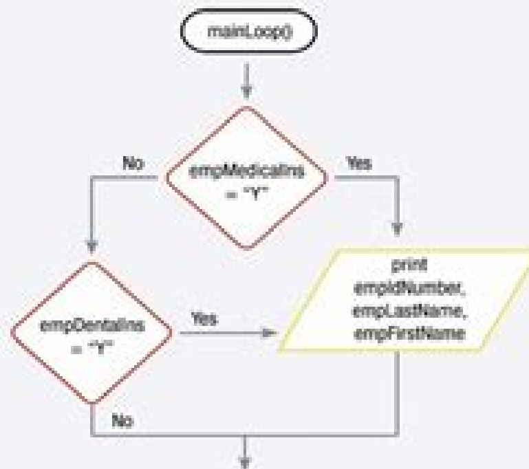
FIGURE 5-21: INCORRECT FLOWCHART FOR mainLoop() MODULE
