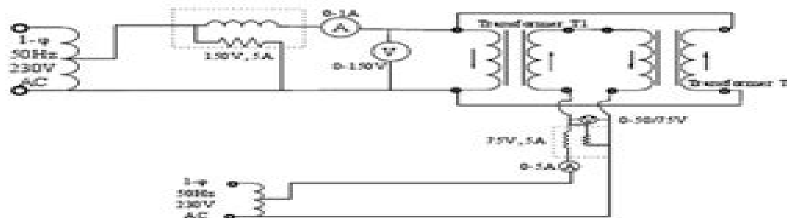
Fig. A. Circuit diagram of Sumpner's back to back test.
