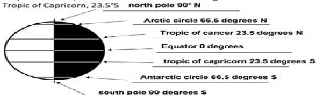
Figure 3.6: The Seven Special Parallels of the Earth. 1
