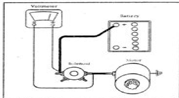
FIGURE 8 (SERVI-CAR)
