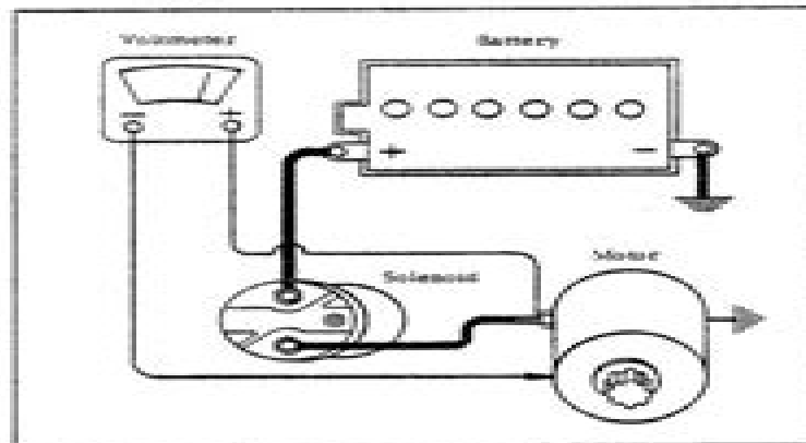
FIGURE 5 (ELECTRA-GLIDE)
