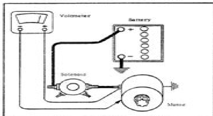
FIGURE 6 (SERVI-CAR)
