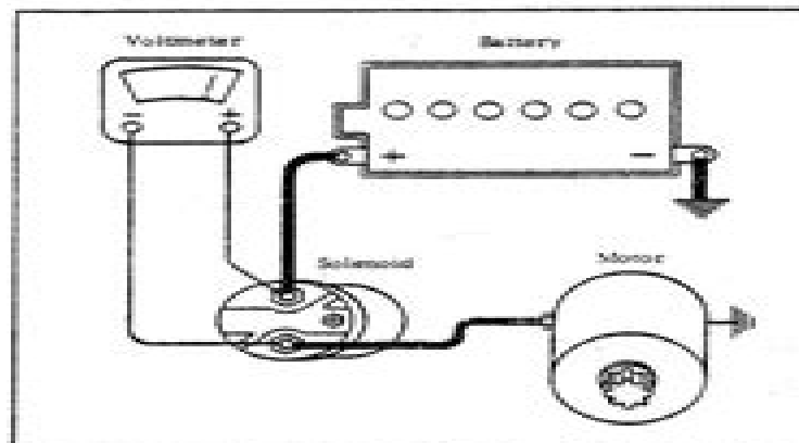
FIGURE 7 (ELECTRA-GLIDE)
