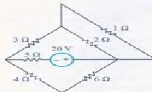
Figure P1.11: Circuit for Problem 1.11.
