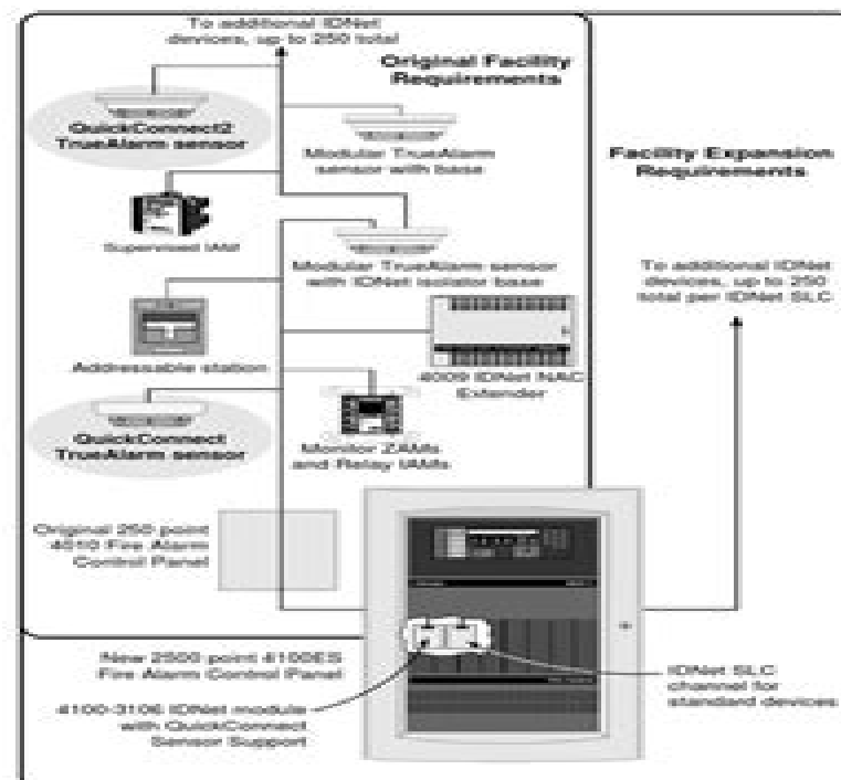
4010 System Expansion using a 4100-3106 IDNet Module
