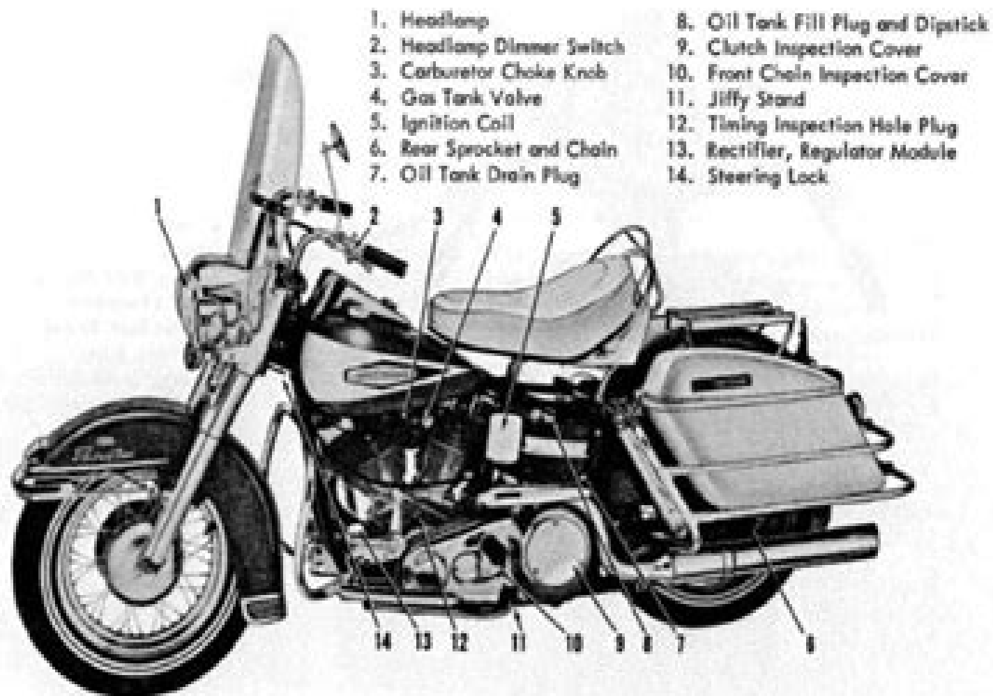
FIGURE 2. LEFT SIDE VIEW
