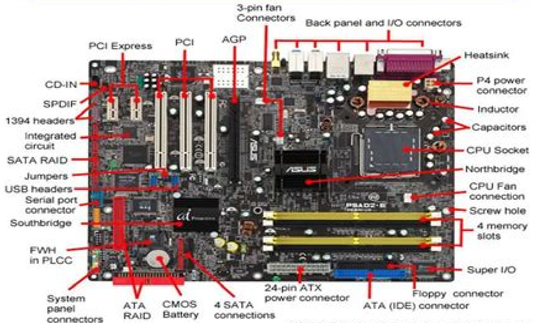
ASUS P5AD2-E Premium Motherboard
