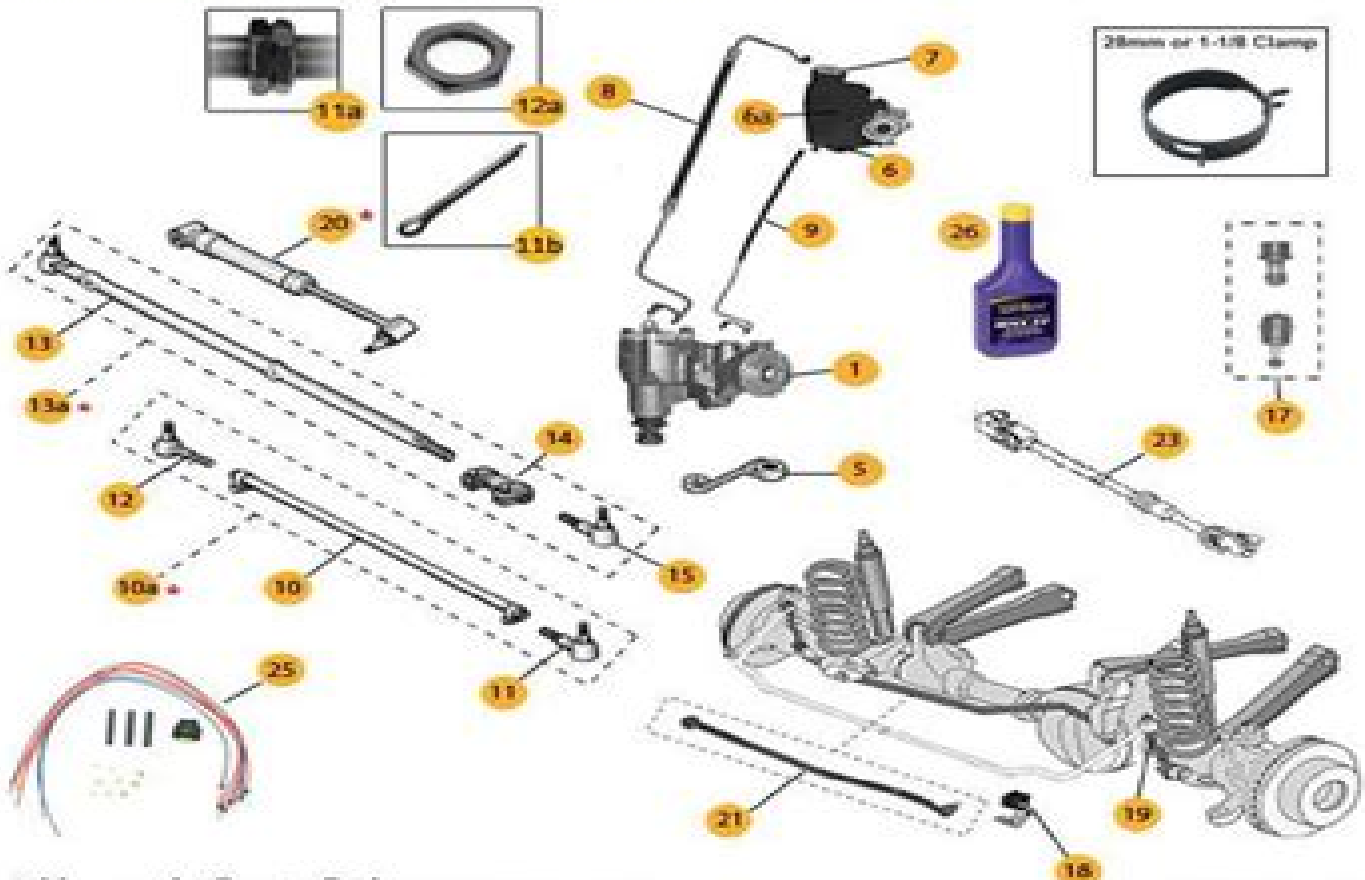
TIE-ROD Heavy duty kit
