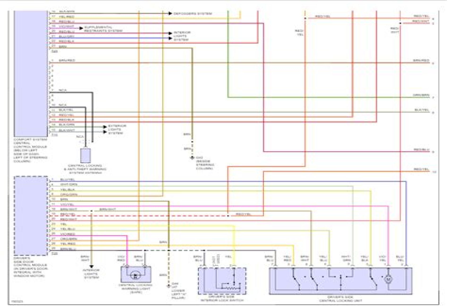
Fig 3: Anti-theft Circuit, Except Convertible (1 of 2)
