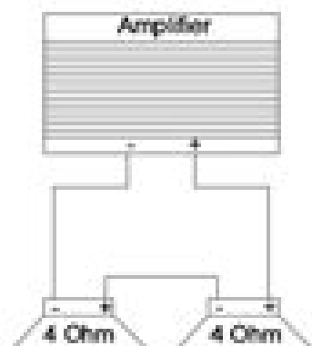
2-4 ohm drivers in series = 8 ohms
