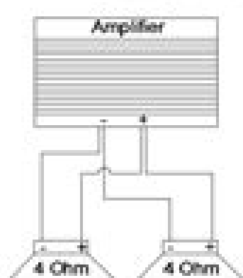
2-4 ohm drivers in parallel = 2 ohms
