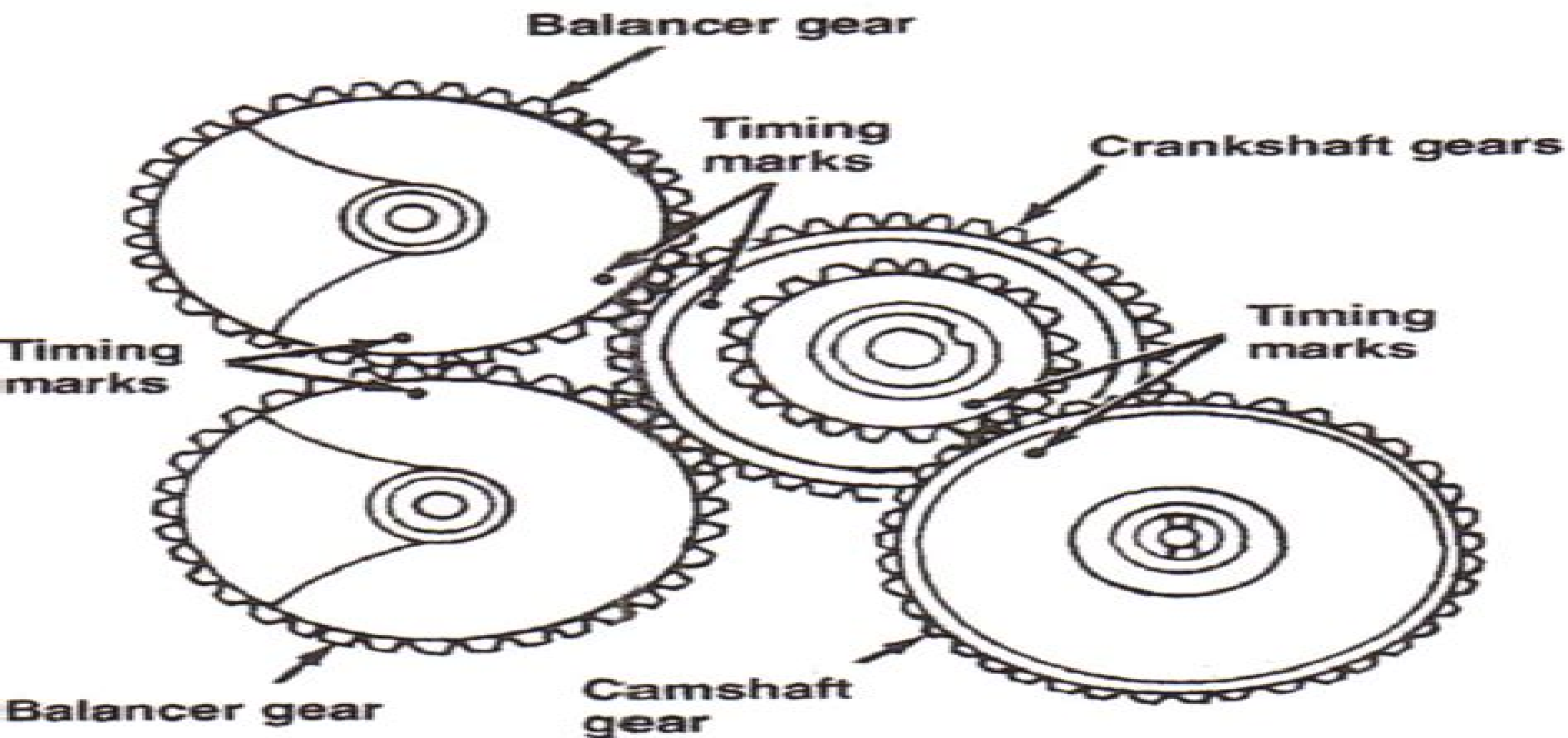
Fig. HE2-9—Drawing showing correct alignment of timing marks on crankshaft, camshaft and balancer shaft gears.
