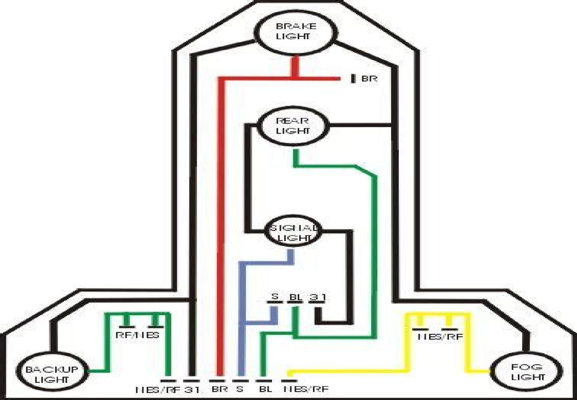
Front View of Harness
