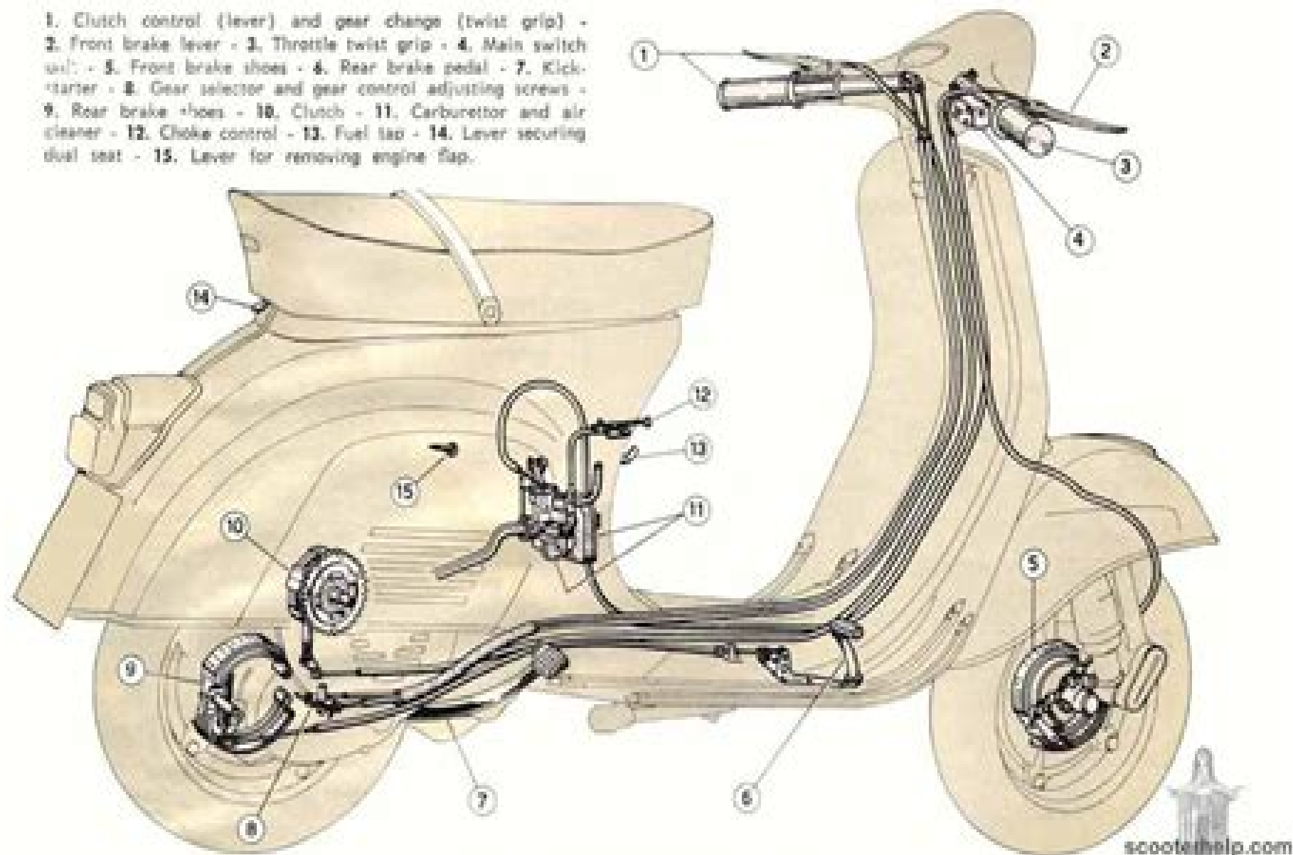
Fig. 2 - Installation of controls and transmission.
