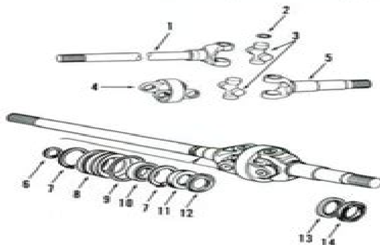
Fig. 7—Exploded view of front-wheel drive axle shaft assembly. Dust seal (12) and oil seal (14) are located in stub axle. Note that L. H. driver axle shaft is shorter than R. H. inner axle shaft.
