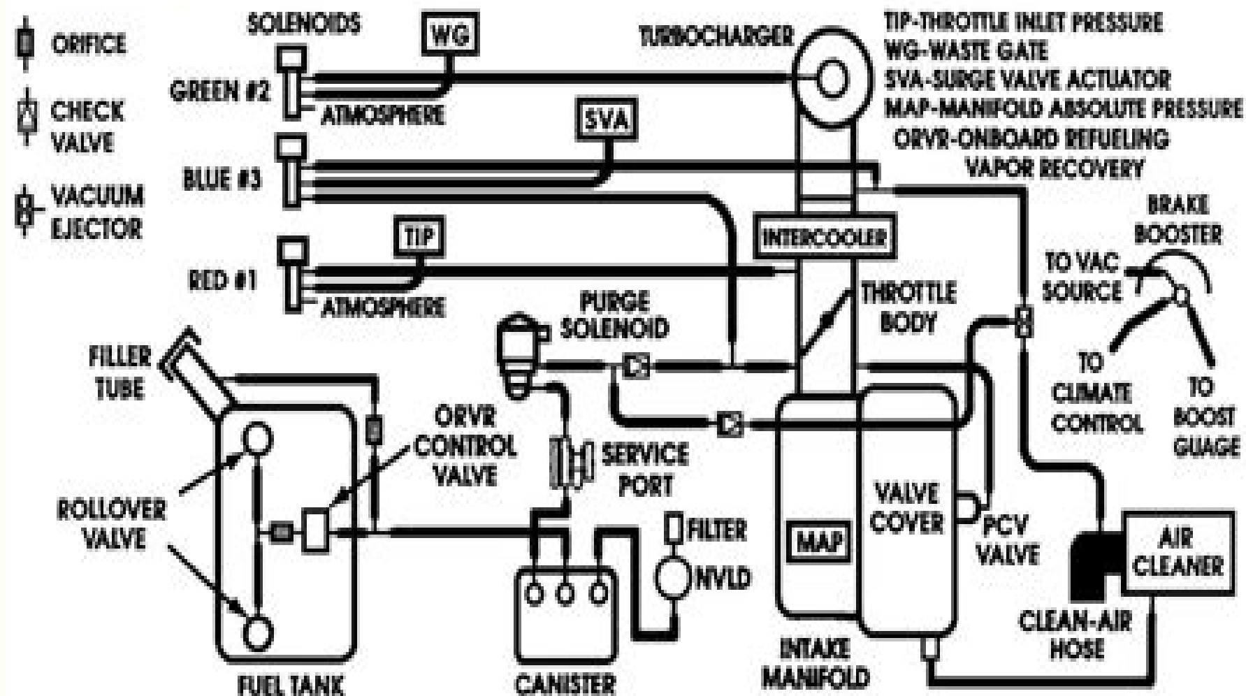
Fig 3. Vacuum Diagram - SRT-4 (2.4L)
