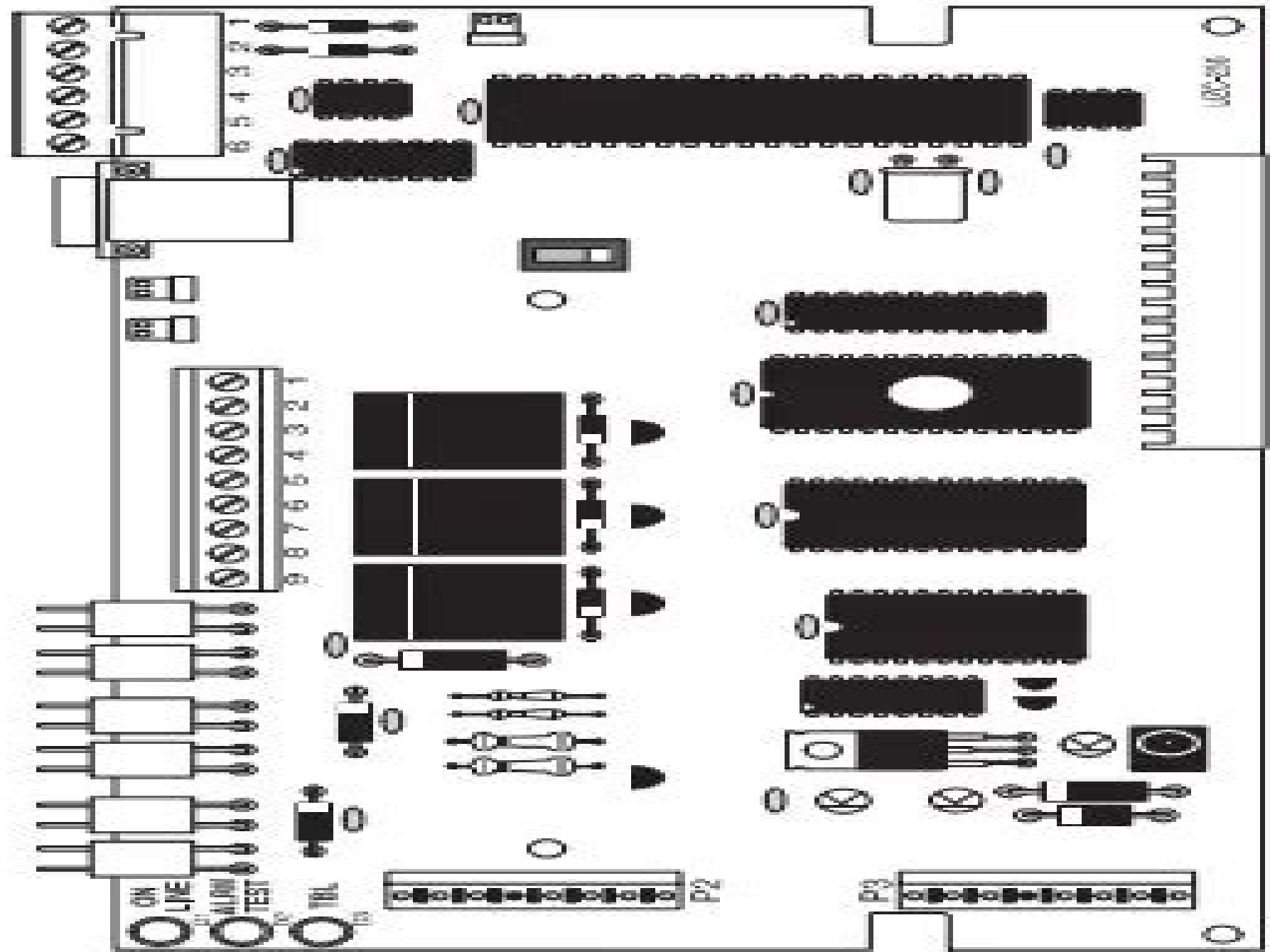
UZC-256 Universal Zone Coder
