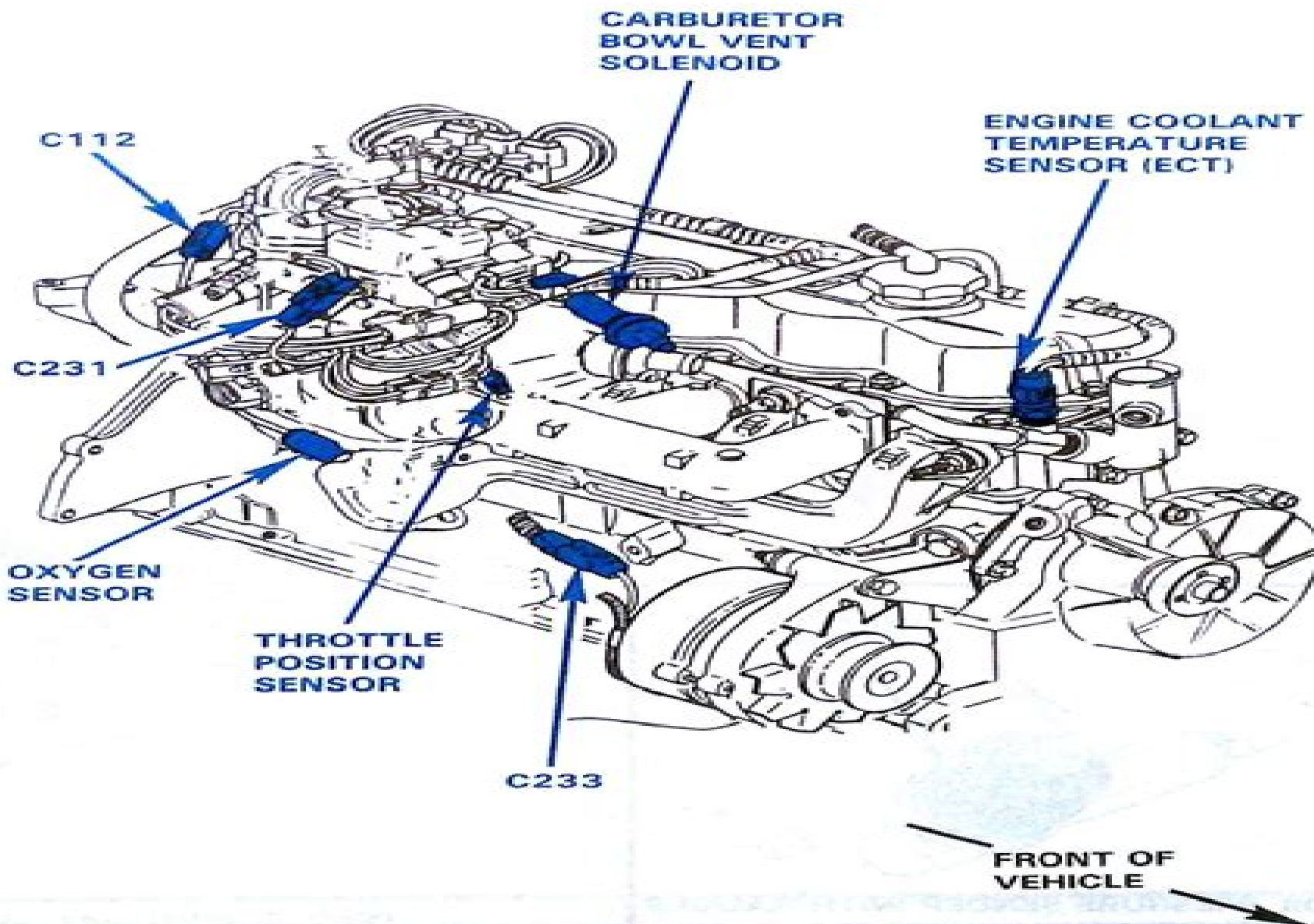
Figure 17 — LH View 4.9L Engine (50 States) Under 8500 lbs. (GVW EEC IV)
