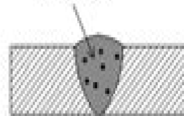
Porosity
