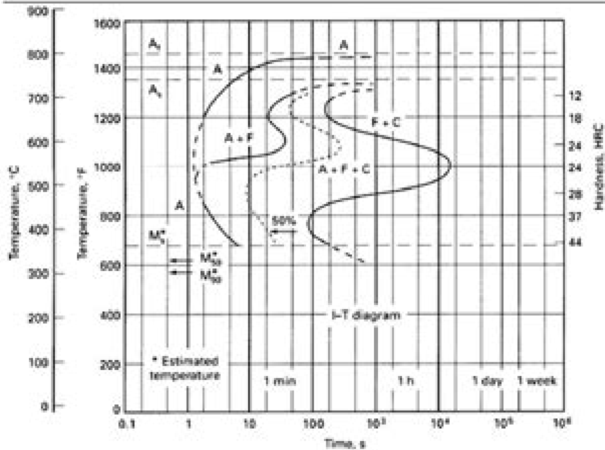
Fig. 35 TTT diagram for 4130 low-alloy steel
