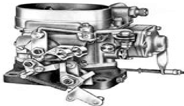
Type 32 PAITA (Downdraught Compound Carburetor)
