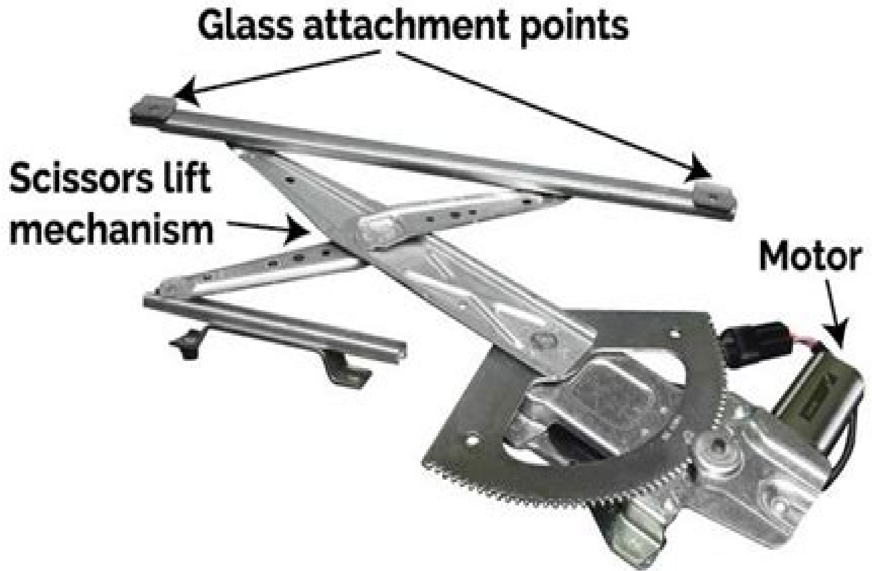
Scissors style window regulator
