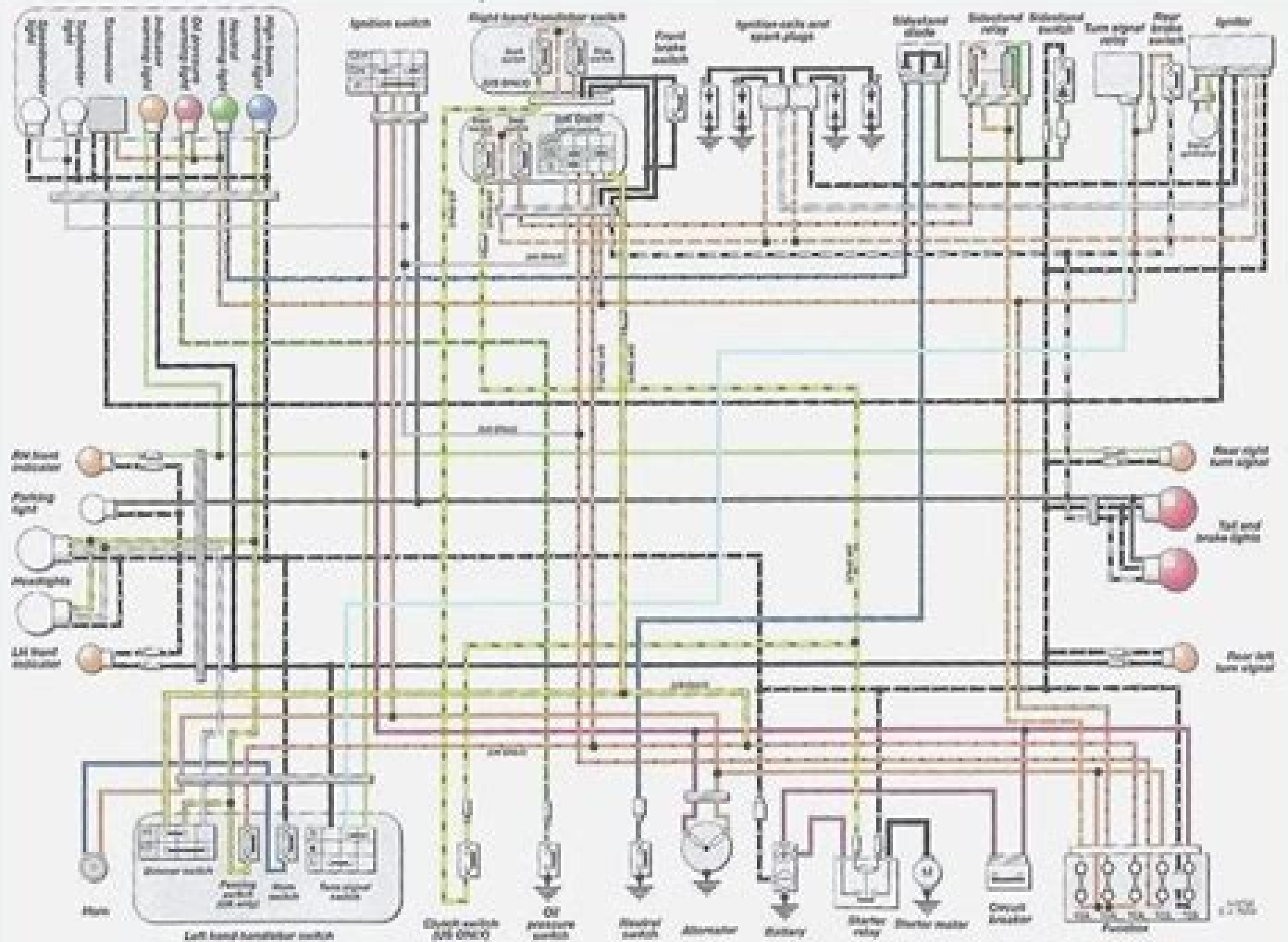
GSX-R750 1991 onwards UK and US models
