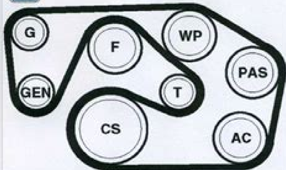
Serpentine belt routing
