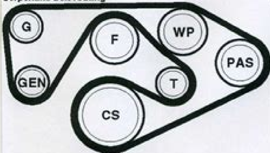
Serpentine belt routing
