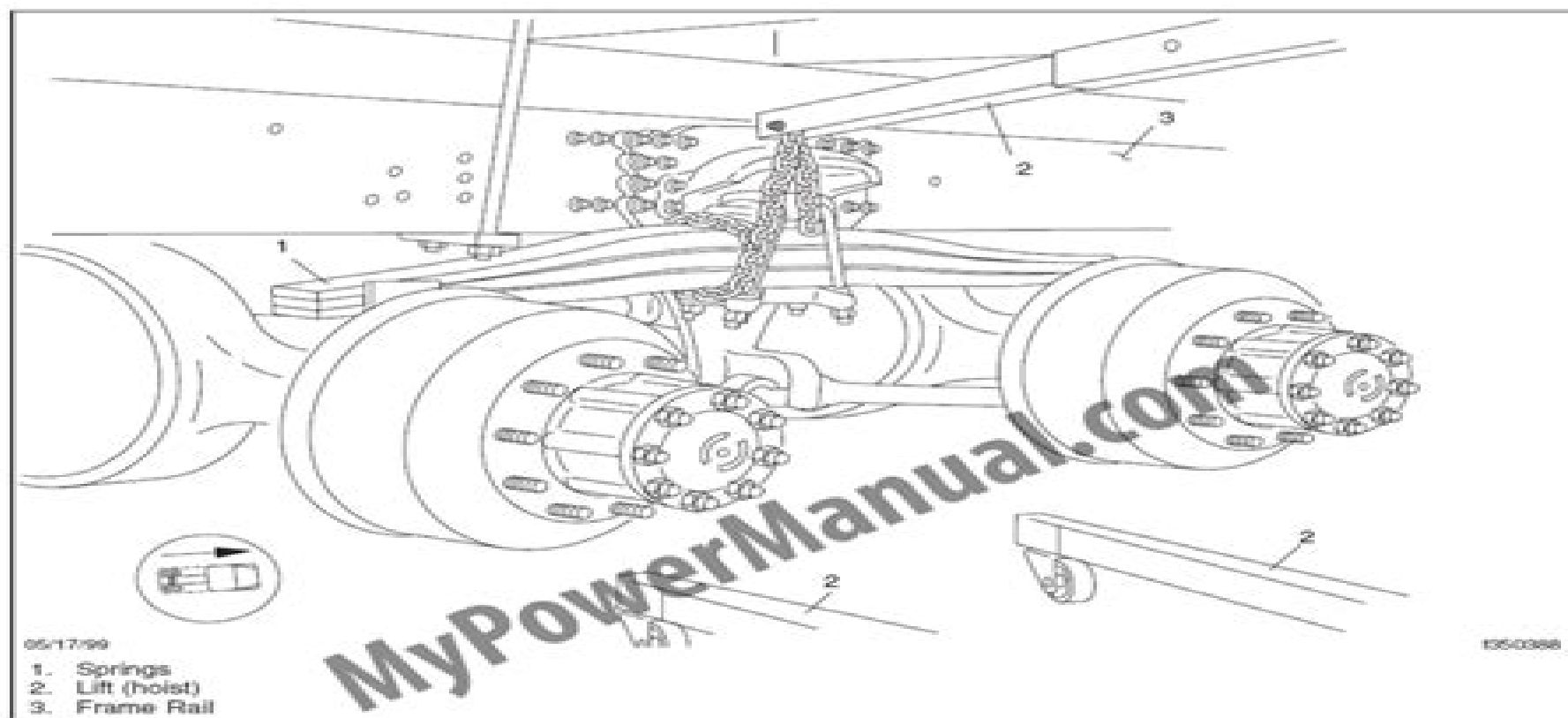
Fig. 2, Leaf Spring Replacement
