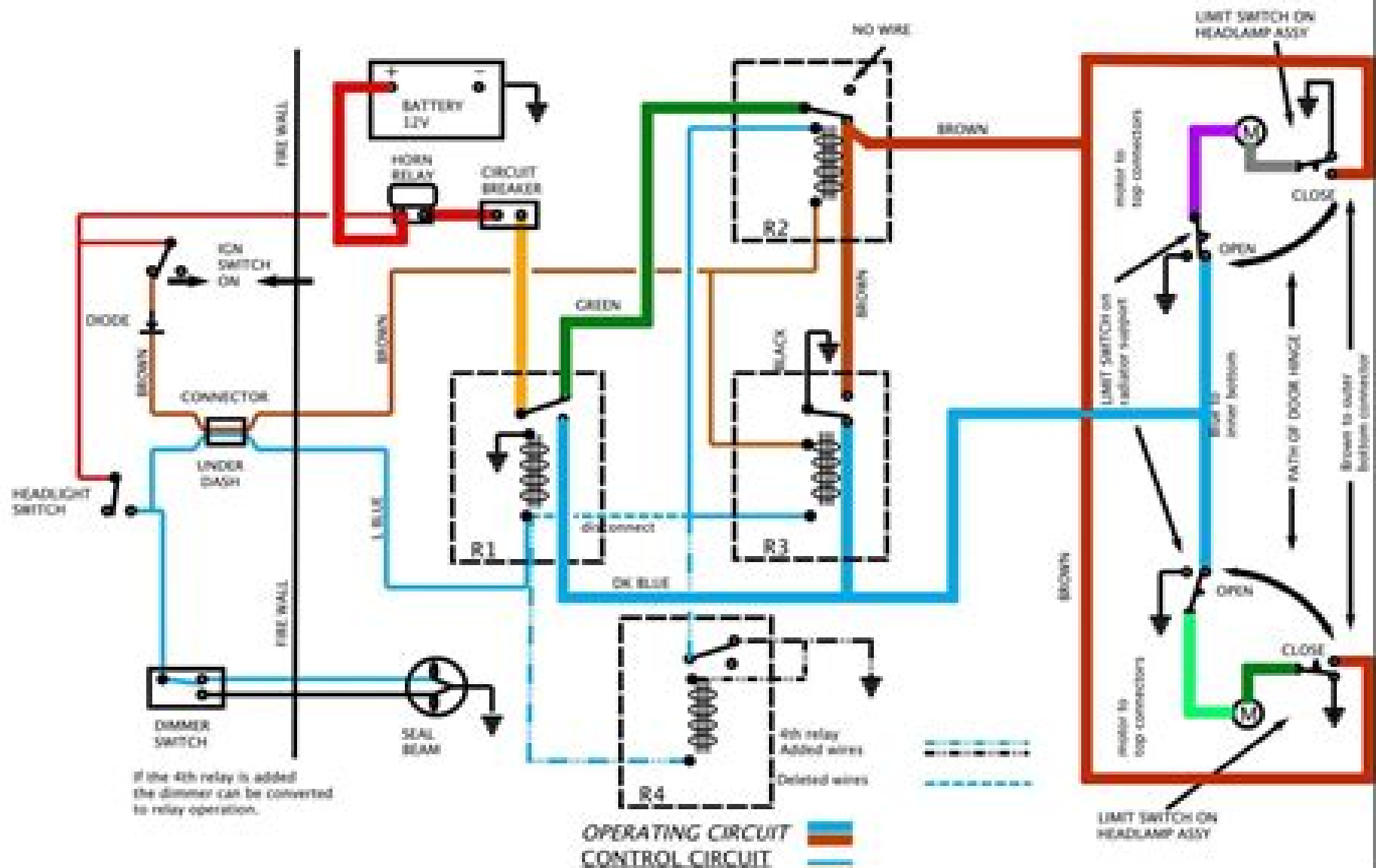
67 CAMARO HEADLAMP DOOR WIRING - LIGHTS OFF, IGN ON, DOORS CLOSED.
