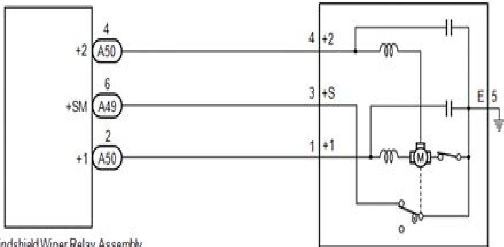
A43 Windshield Wiper Motor Assembly
