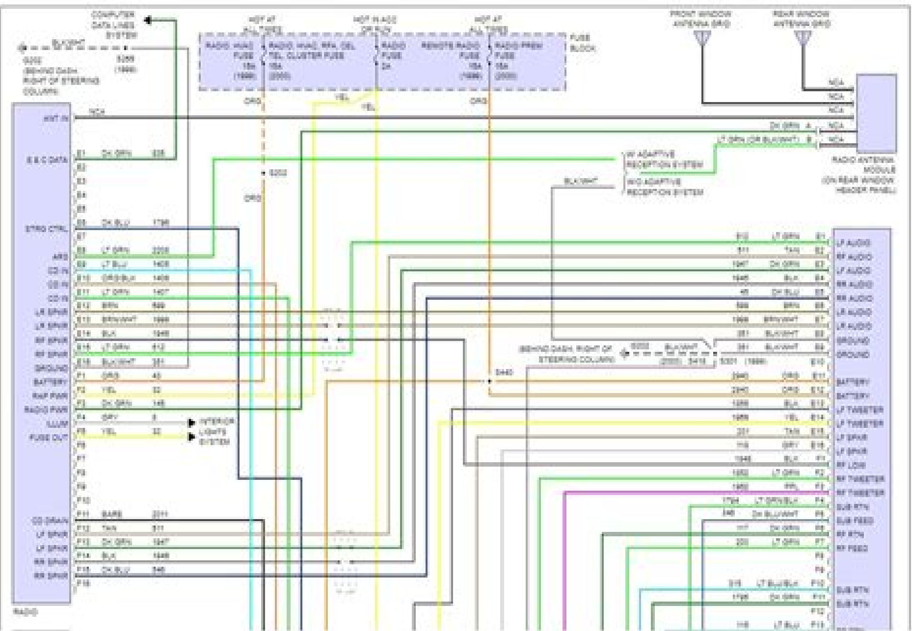
Fig. 1. Radio Circuits, VHF Amplifier
