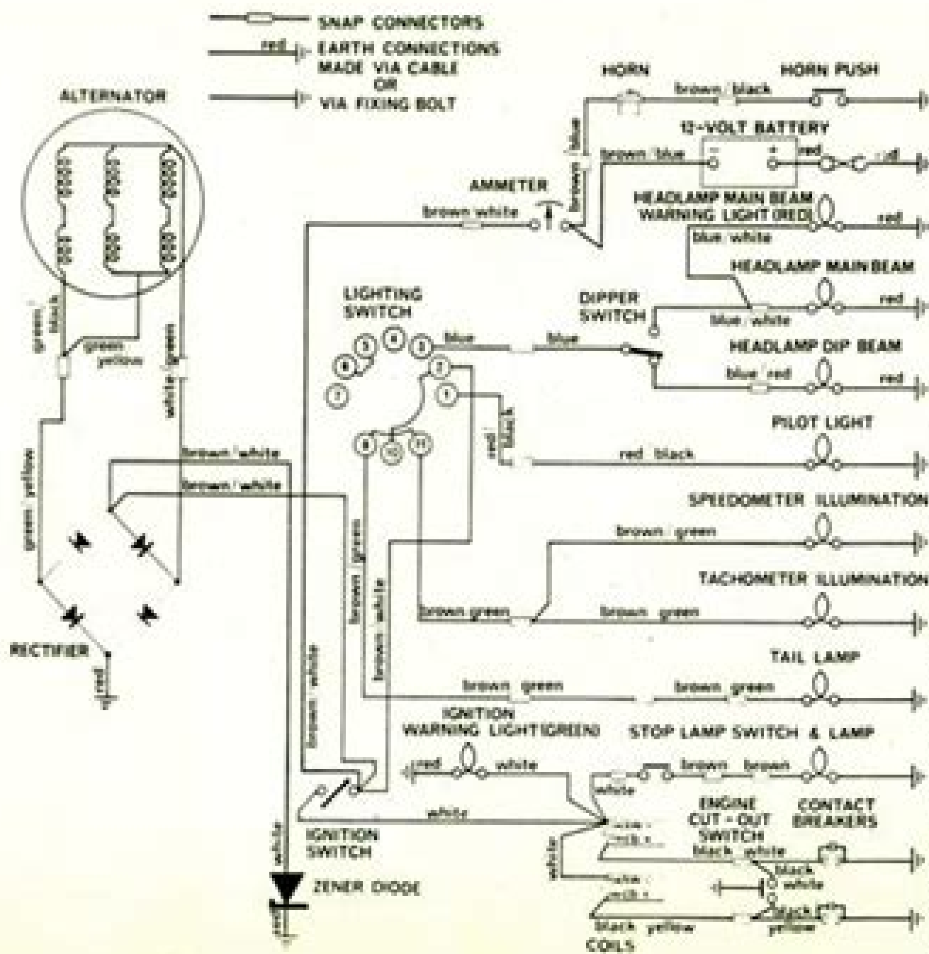
Fig. H13. Wiring diagram—Coil ignition 12 volt models with separate headlamps from engine number DU 3407 (Humber) Note. The main beam warning lamp (where fitted) is connected to the headlamp main beam wire (blue/white) by a double snap connector. The ignition warning lamp is connected to an ignition coil by a white wire incorporated in the wiring harness.
