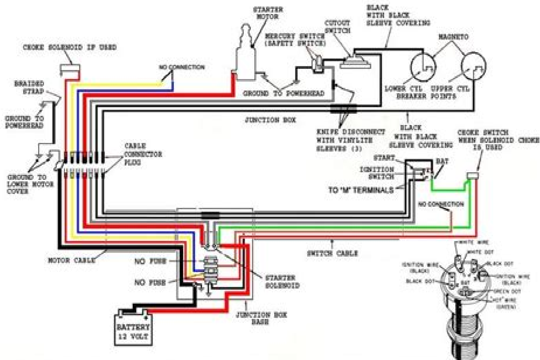
WIRING DIAGRAM FOR 1958-61 35 AND 40 HORSEPOWER MODELS (WITHOUT GENERATOR KIT)
